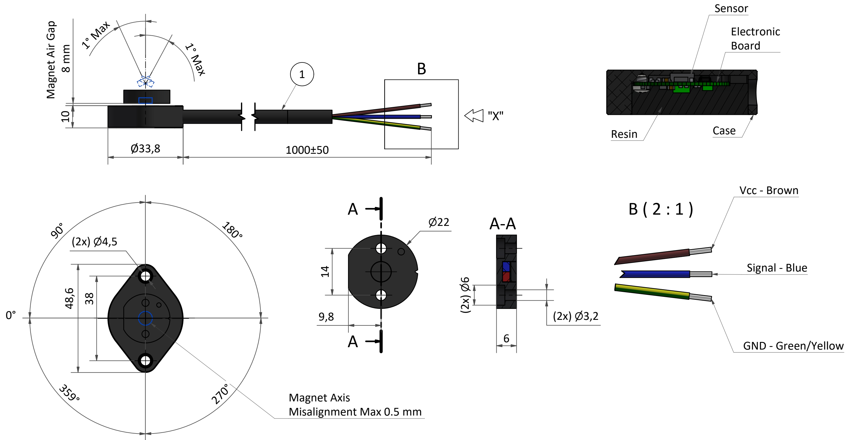
The picture represents the Alignment between Sensor and Magnet Carrier at the 0° position
