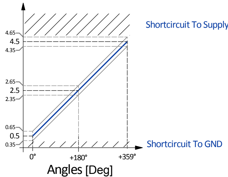
Signal 2 (V) @Vin = 10÷30V
