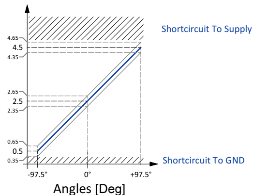
Signal 2 (V) @Vin = 5V
