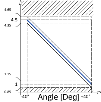
Signal 2 (V) @Vin = 5V
