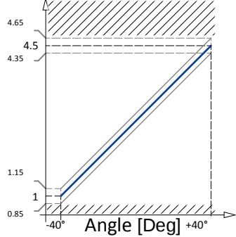
Signal 1 (V) @Vin = 5V
