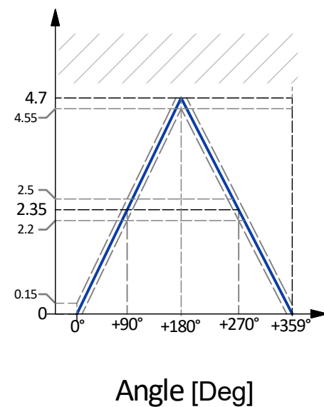
Signal (V) @Vin = 5V
