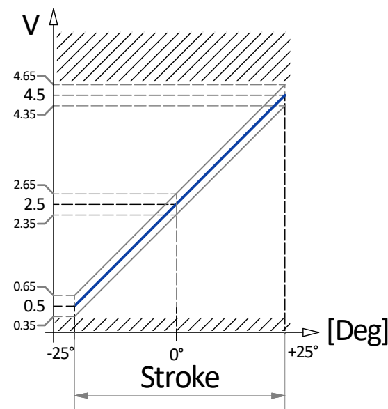
Output Signal (V) @Vcc = 10÷30V
