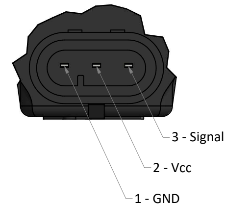
Details "B" ( 2 : 1 )
