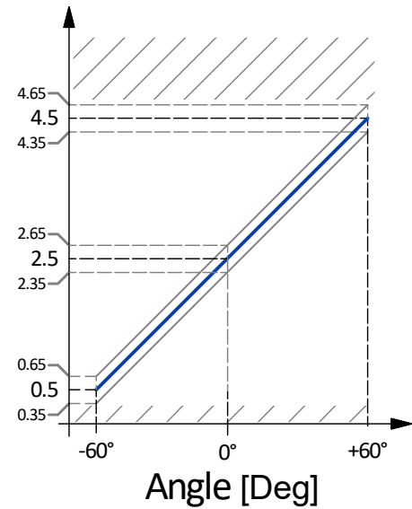
Signal (V) @Vin = 5V
