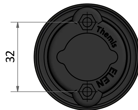
View from "Y"
