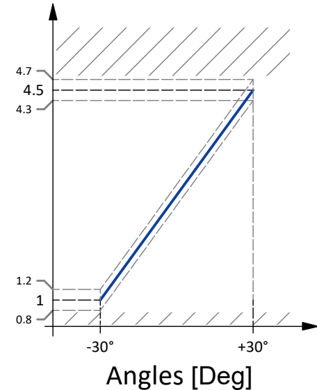
Signal 1 (V) @Vin = 5V
