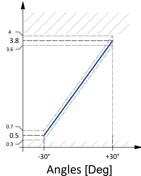
Signal 2 (V) @Vin = 5V
